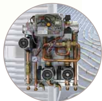
Kit impianto misto universale MS IN (1 AT - 2 BT)
